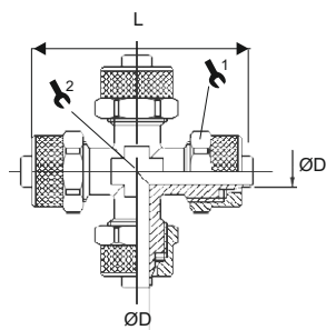
CROSS UNION / CROIX / CROCE INTERMEDIO
