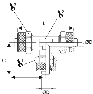
UNION TEE / T / T INTERMEDIO
